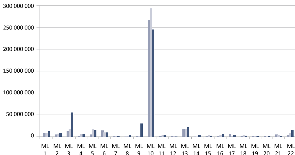
Chart 3: 2013–2015 actual export value as per the Common Military List categories (in EUR)
