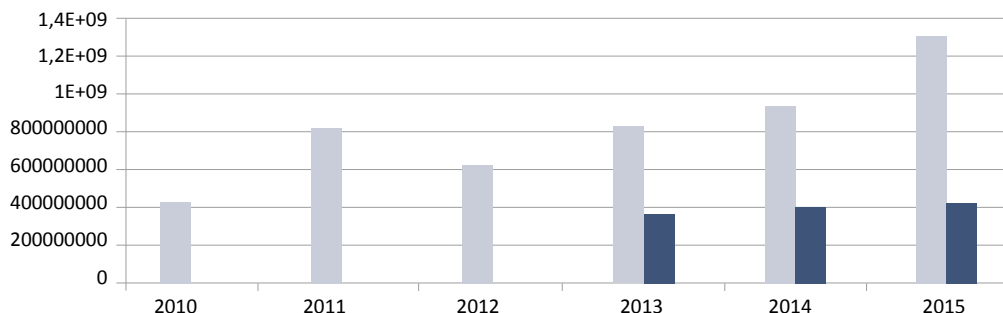
Chart 2: Changes in the total value of licenses issued in the years 2010–2015 and the value of actual exports in the years 2013–2015
