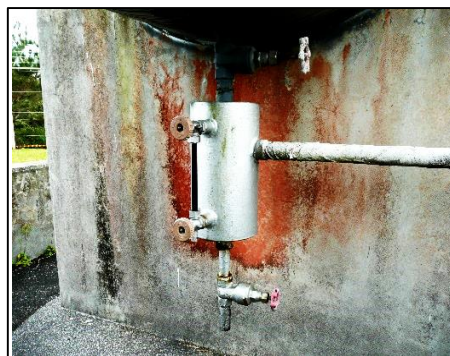
Corrosion of fuel tank for equipment facility
